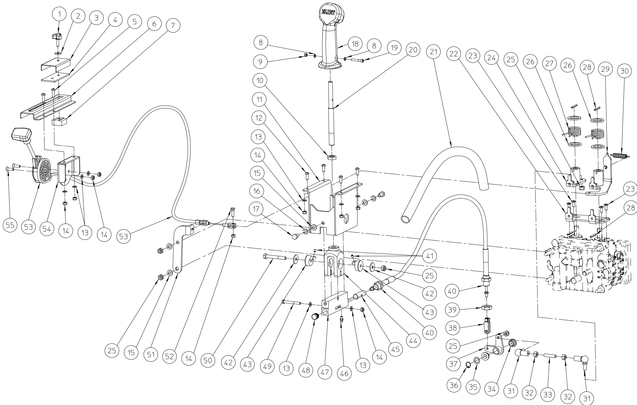
ELIET ECOCURE ZR -- CONTROL LEVER
