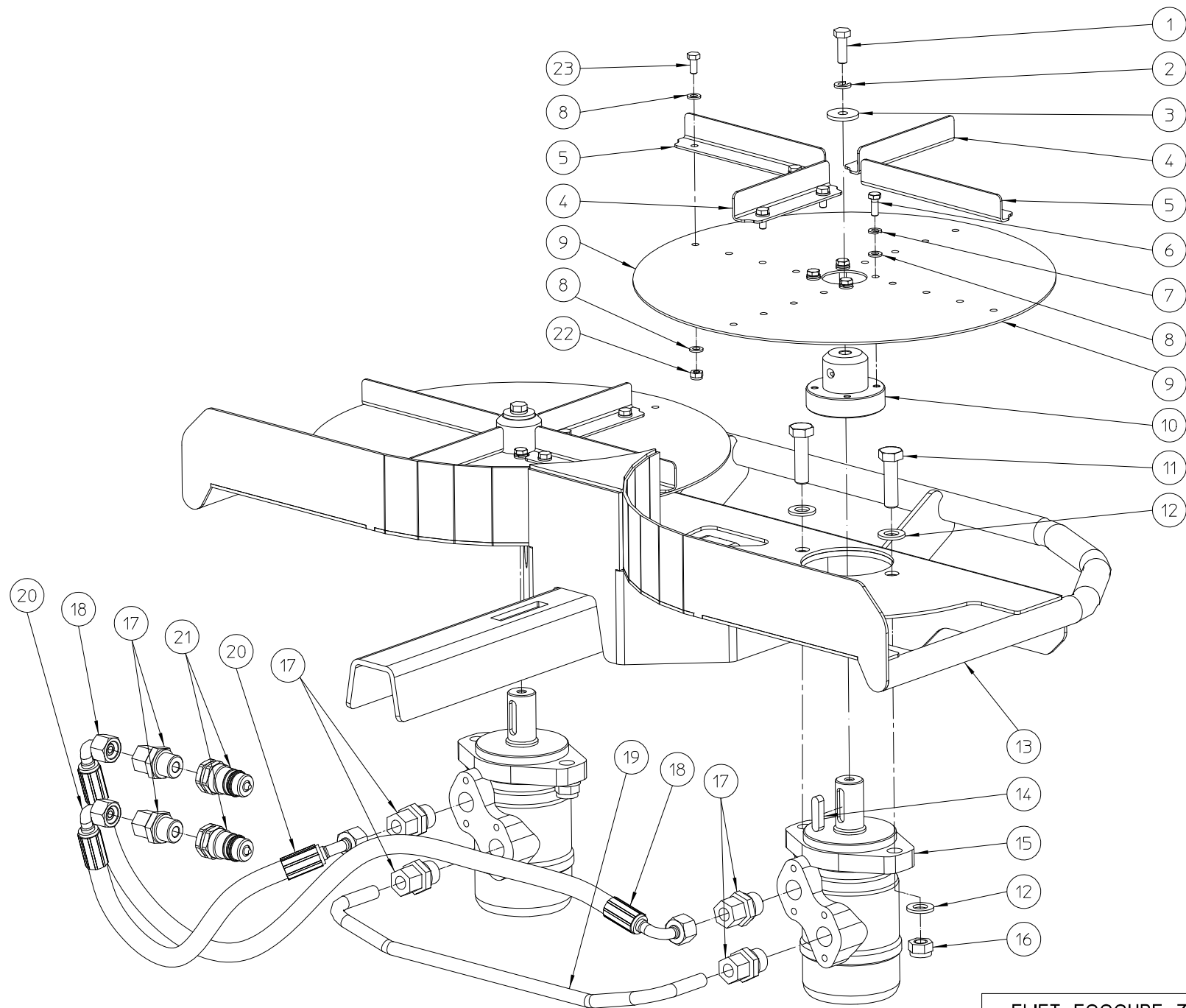
ELIET ECOCURE ZR -- DISC SPREADER
